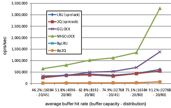
Fig. 8. Throughputs obtained when varying buffer capacity and workload distributions.
