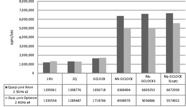
Fig. 13. Experiment on X86-64 architecture (8 threads).
