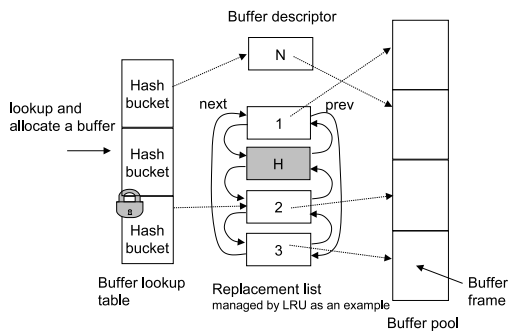
Fig. 1. Typical organization of a buffer manager.
