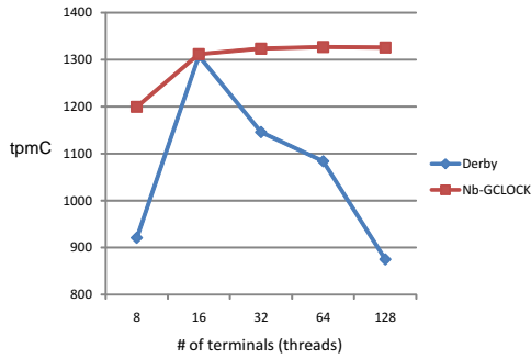
Fig. 15. Comparison of tpmC between Nb-GCLOCK and Derby's CLOCK.
