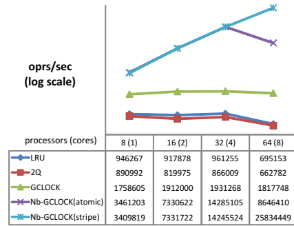
Fig. 10. Scalability to processors when pages are resident in memory.
