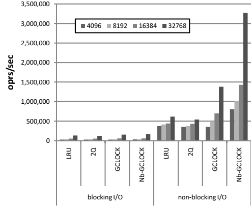
Fig. 9. Comparison between “blocking I/O” and “non-blocking I/O”.
