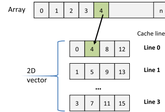
Fig. 14. Expressing an array as a two-dimensional vector.
