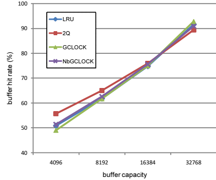
Fig. 7. Relationship between buffer capacity and buffer hit rate (64 threads).
