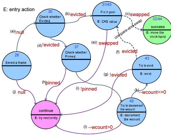
Fig. 5. State transitions in clock-sweep.
