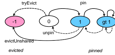
Fig. 2. State machine of a pinning instance.
